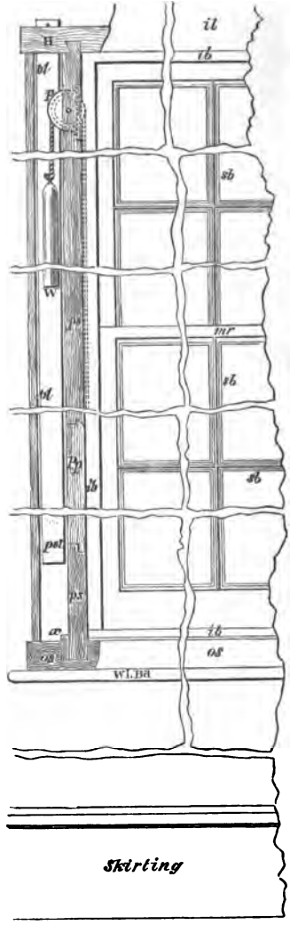
Elevation of part of Interior (1/2) (the inside lining having been removed)
